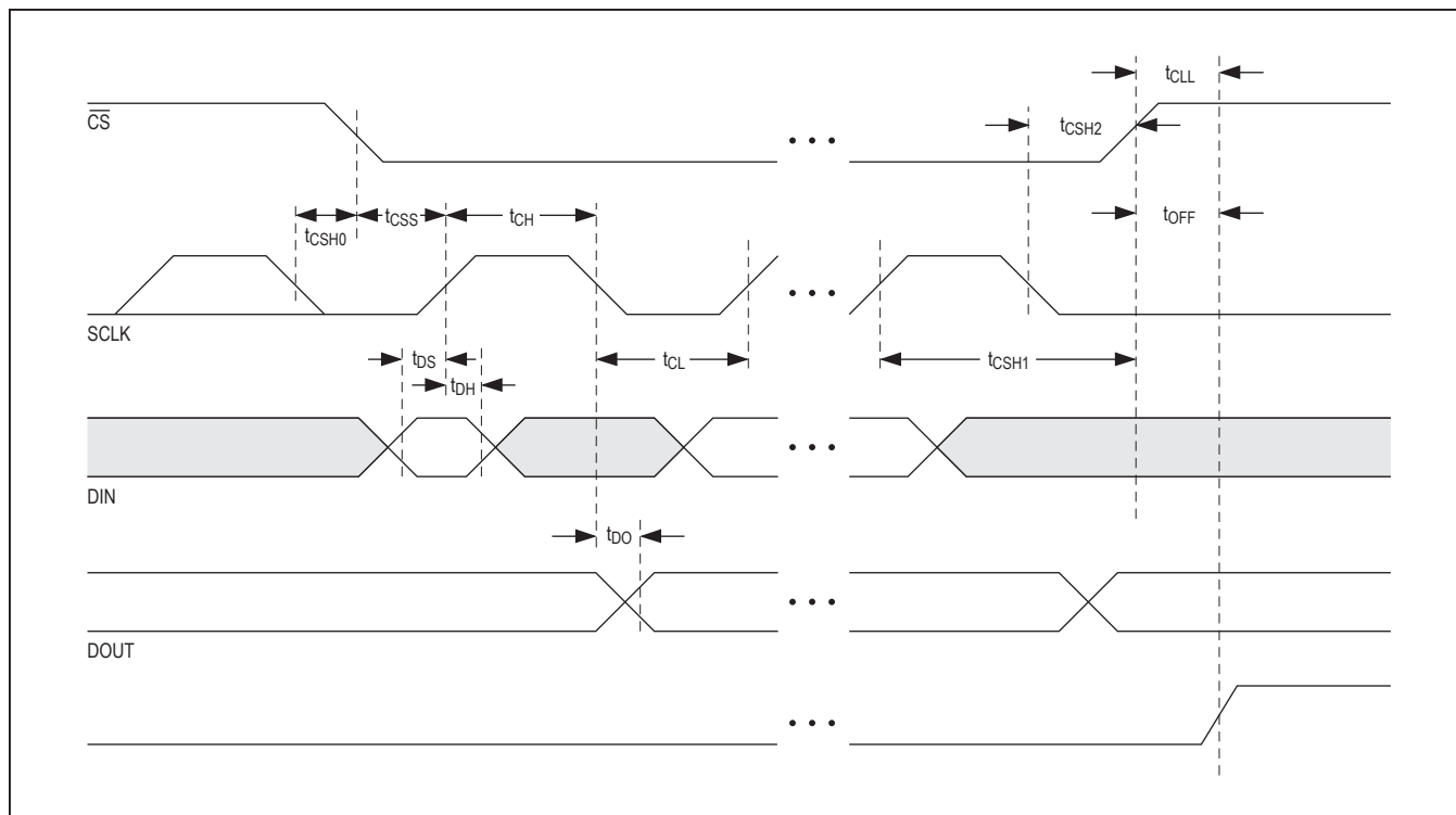
Figure 1. Timing Diagram
