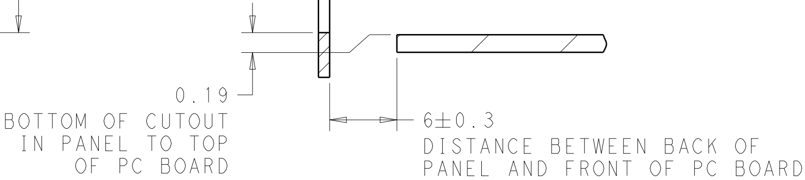
SECTION U-U
