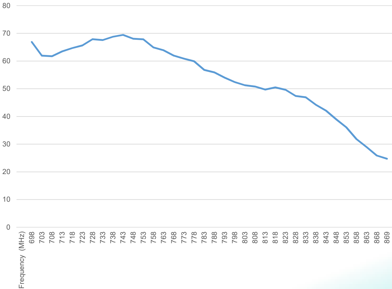
ICEFIN698/869DMN Efficiency (%)
