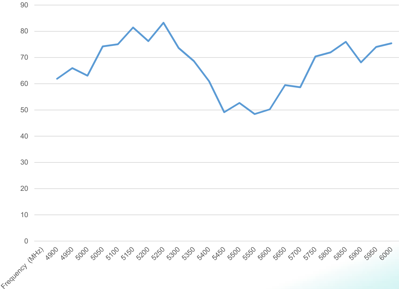
ICEFIN49DMN Efficiency (%)
