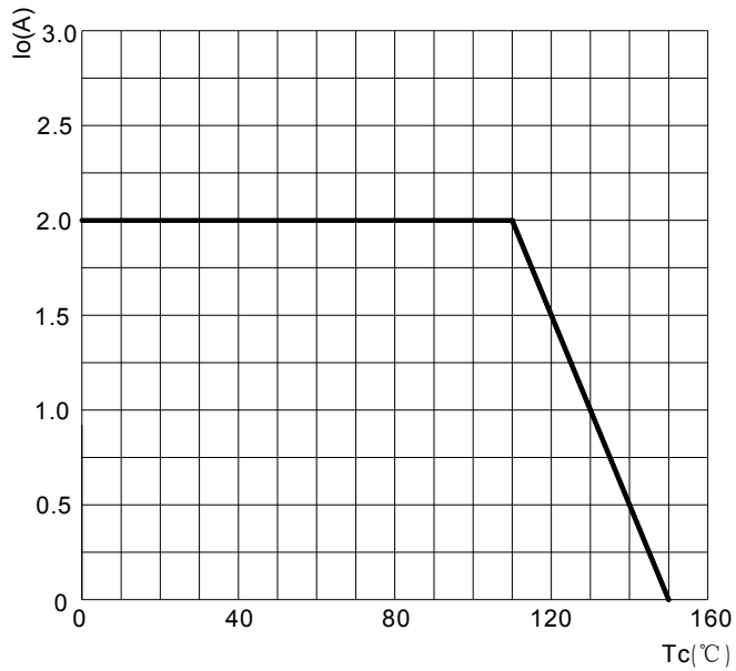
FIG1:Io-Tc Curve
