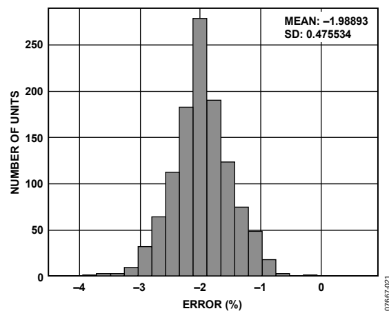
Figure 21. Typical Uncalibrated Accuracy for the Battery Channel (25°C)
