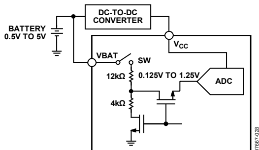
Figure 28. Block Diagram of Battery Measurement Circuit
