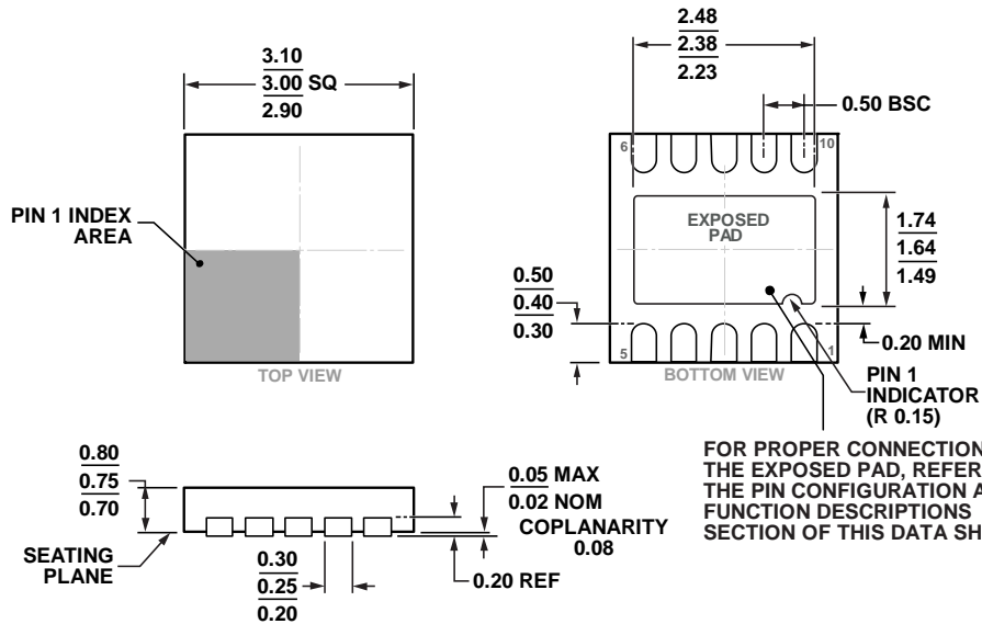
Figure 49. 10-Lead Frame Chip Scale Package [LFCSP_WD] 3 mm x 3 mm Body, Very Thin, Dual Lead (CP-10-9) Dimensions shown in millimeters
