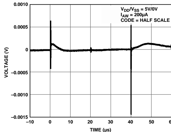
Figure 35. Digital Feedthrough
