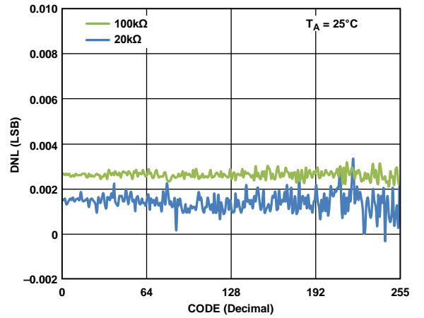
Figure 23. R-DNL in Normal Mode vs. Code vs. Nominal Resistance (AD5271)
