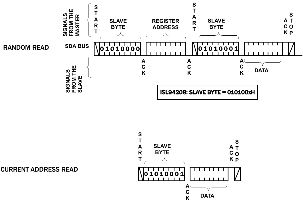
FIGURE 27. READ SEQUENCE
