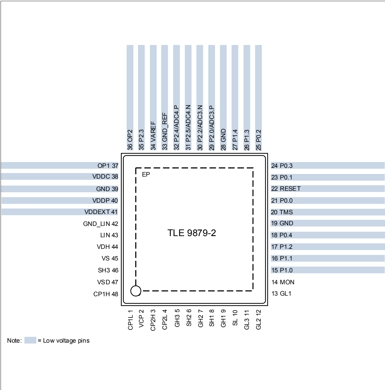
Figure 3 Device Pinout
