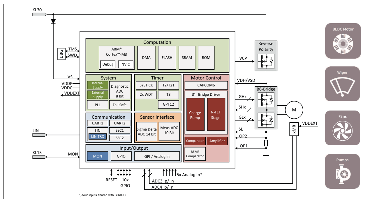
Figure 1 TLE9879-2QXA40 simplified application diagram
