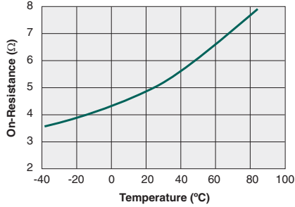
Typical On-Resistance vs. Temperature ( I_F=0mA, I_L=150mA )
