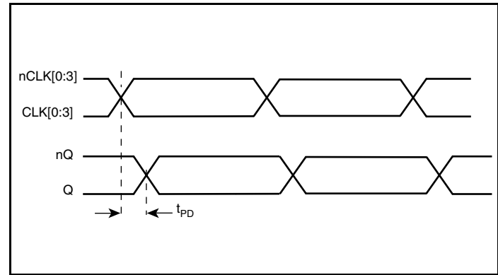
Propagation Delay
