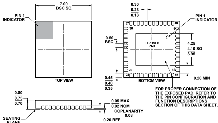
Figure 78. 48-Lead Lead Frame Chip Scale Package [LFCSP_WQ] 7 mm × 7 mm Body, Very Thin Quad (CP-48-5)
