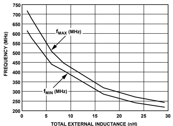
Figure 37. Direct RF Output vs. Total External Inductance
