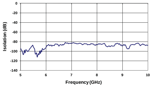
Isolation (5-10 GHz)
