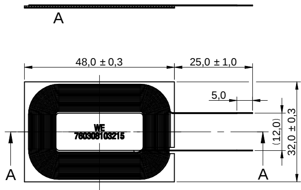
sectional drawing A-A
