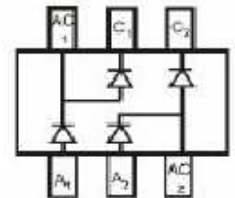
BAT54BR
