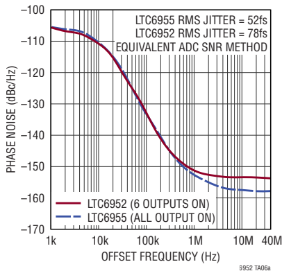
LTC6955 vs LTC6952 4GHz Phase Noise
