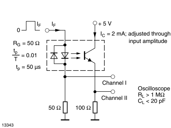
Fig. 3 - Test Circuit, Non-Saturated Operation
