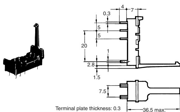
P2R-08P (2-pole)
