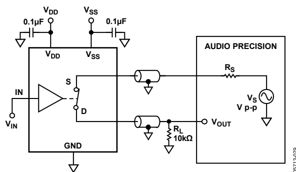
Figure 41. THD + N
