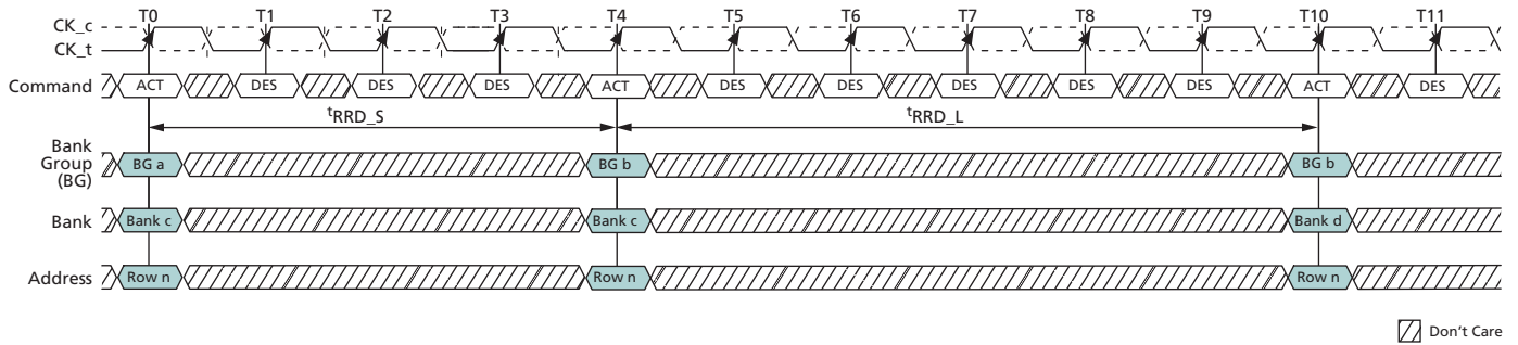
Figure 117: t_{RRD} Timing
