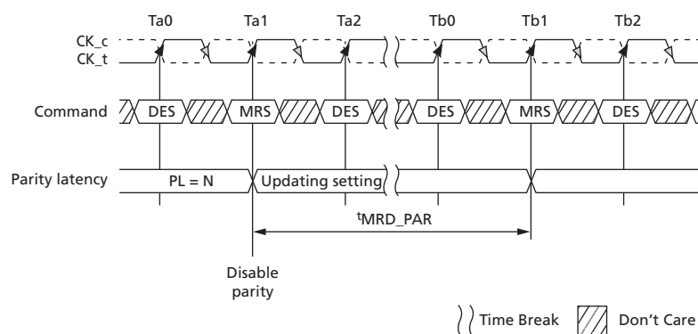
Figure 55: Parity Exit Timing Example – t_{MRD\_PAR}
