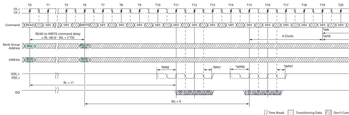
Figure 140: READ (BC4) OTF to WRITE (BC4) OTF with 1 st CK Preamble in Same or Different Bank Group
