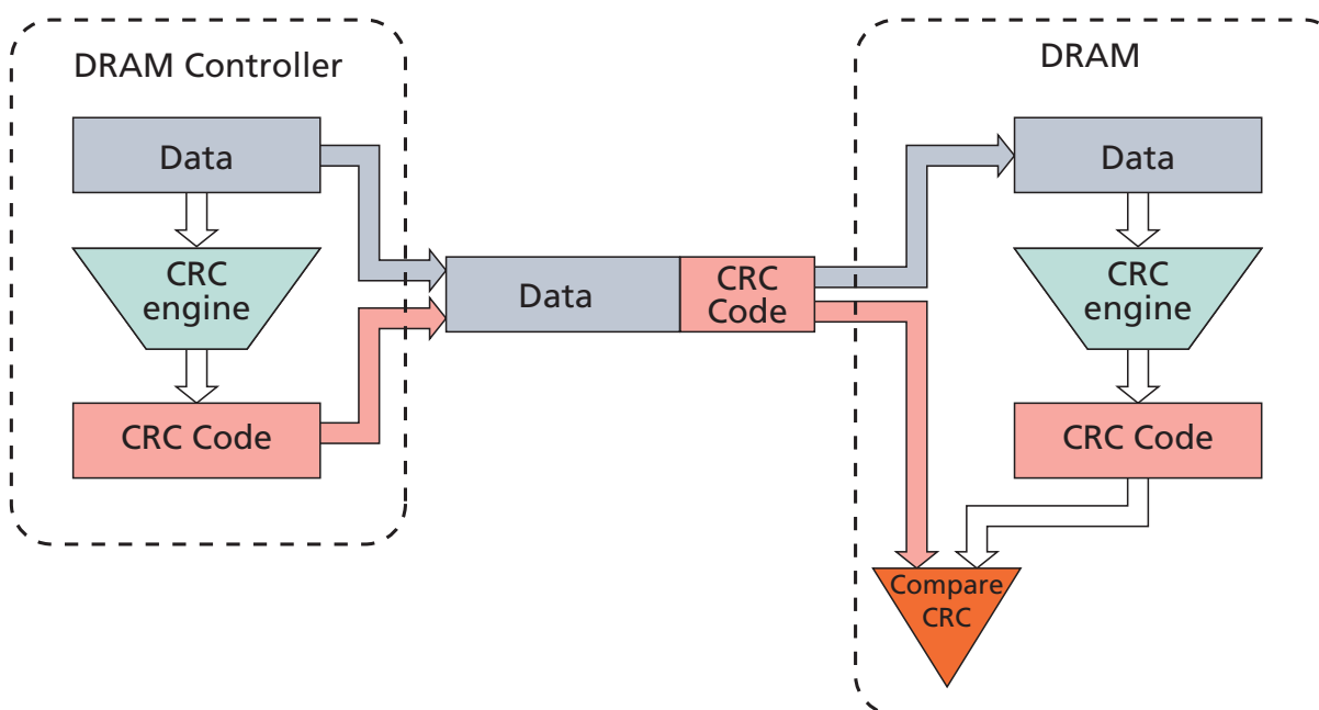
Figure 103: CRC Write Data Operation
