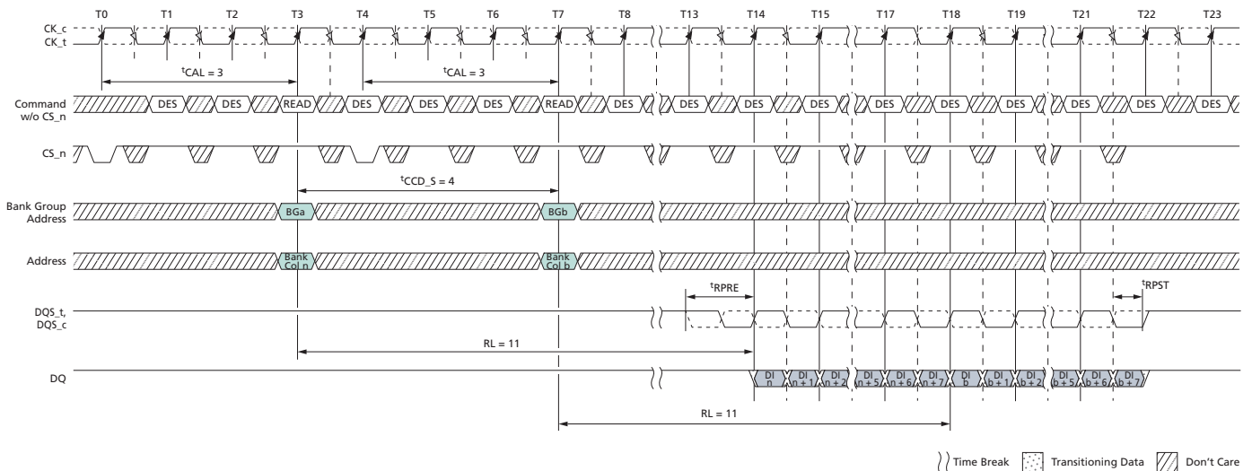
Figure 158: Consecutive READ (BL8) with CAL (3 t CK) and 1 t CK Preamble in Different Bank Group
