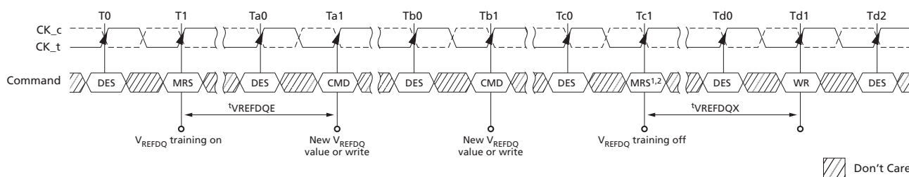
Figure 64: V REFDO Training Mode Entry and Exit Timing Diagram
