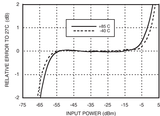
LOGOUT Error vs. Input Power, Normalized [2], F_{in} = 1900 MHz
