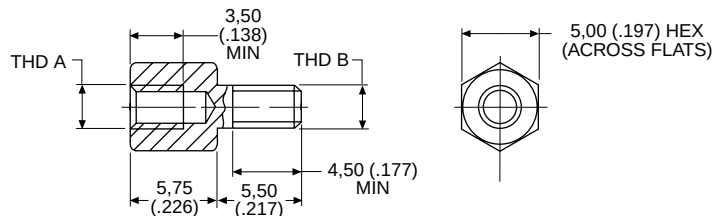
Jackpost
