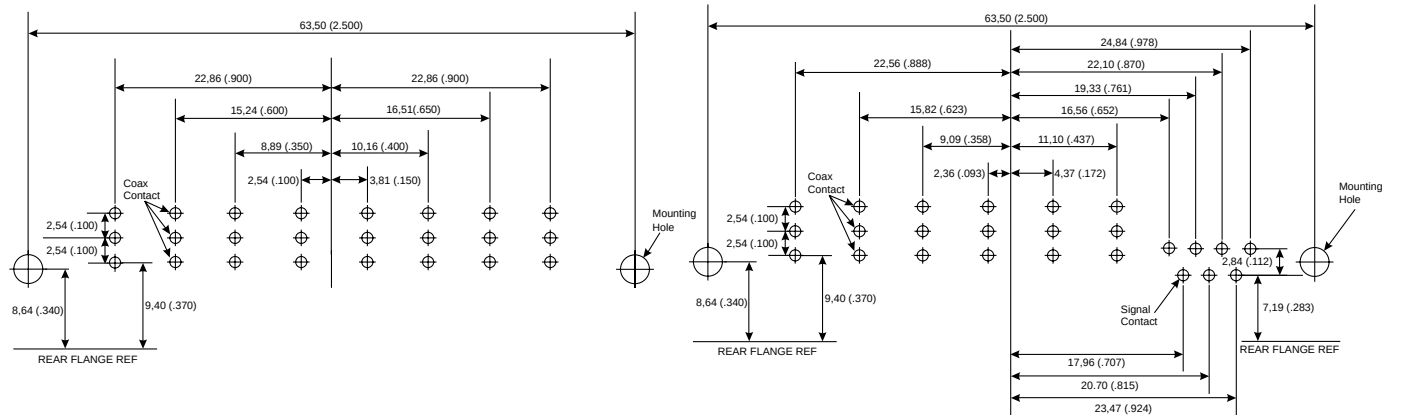
Shell Size C 8W8 0 #20 8 #8 Contact Arrangement No. of Size 20 Cavities No. of Size 8 Cavities C 13W6 7 #20 6 #8
