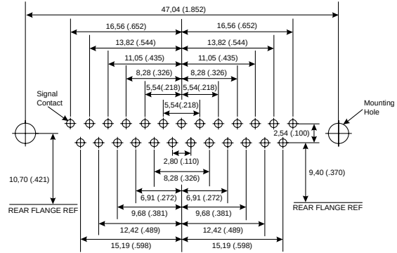
25 Contacts
