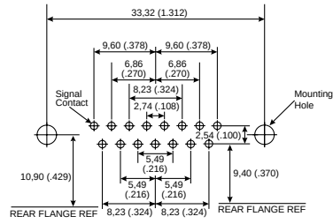
15 Contacts
