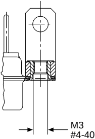
Plastic Bracket with Captive Nut (1ATN/1AVN)
