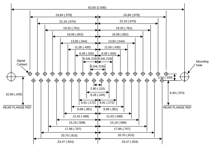
37 Contacts
