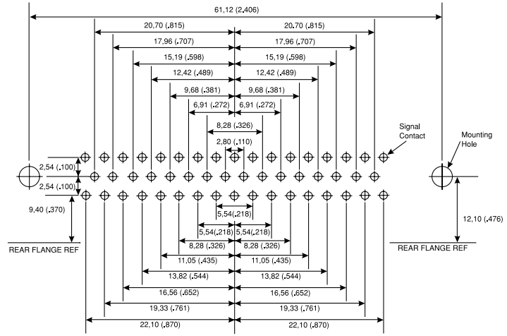
50 Contacts
