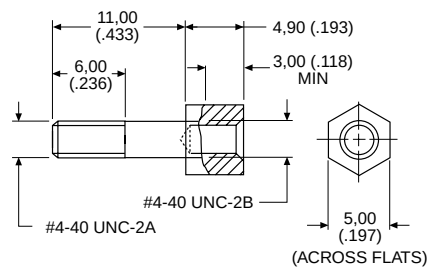
Jackpost
