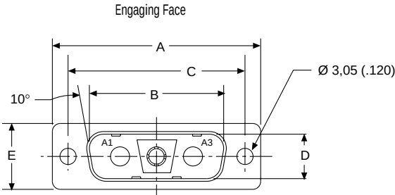
Keyed Configuration
