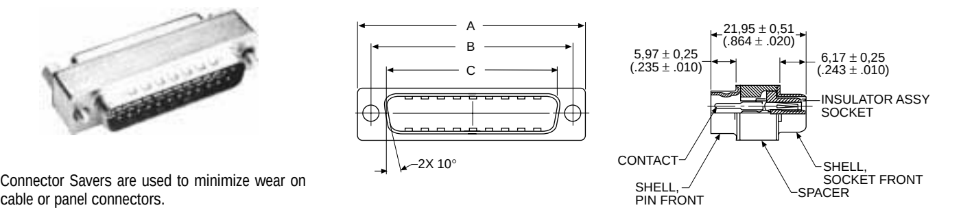
Connector Saver
