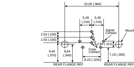
Shell Size Contact Arrangement No. of Size 20 Cavities No. of Size 8 Cavities E 5W1 4 #20 1 #8
