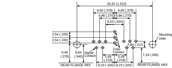
Shell Size Contact Arrangement No. of Size 20 Cavities No. of Size 8 Cavities A 11W1 10 #20 1 #8
