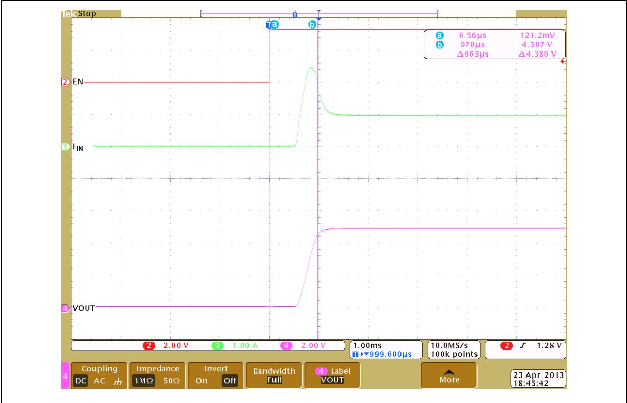
Figure 20. Turn-on response ( R_{ILIM} = 20\text{ k}\Omega , R_{LOAD} = 5\text{ }\Omega , C_{LOAD} = 150\text{ }\mu\text{F} )
