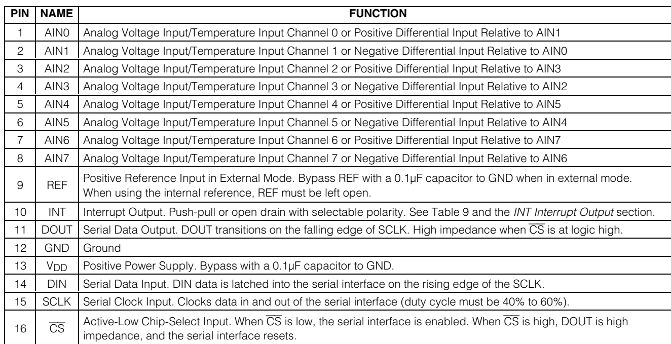
Pin Description
