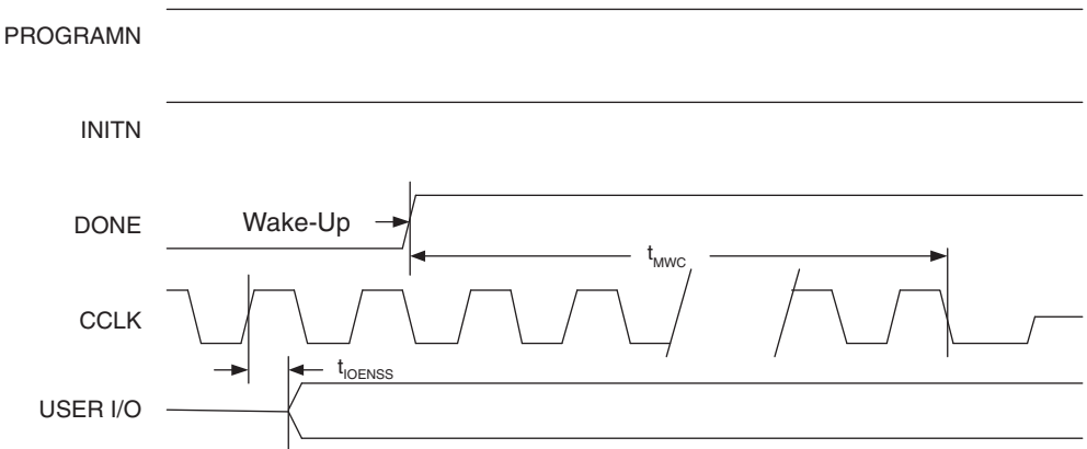
Figure 3-23. Wake-Up Timing
