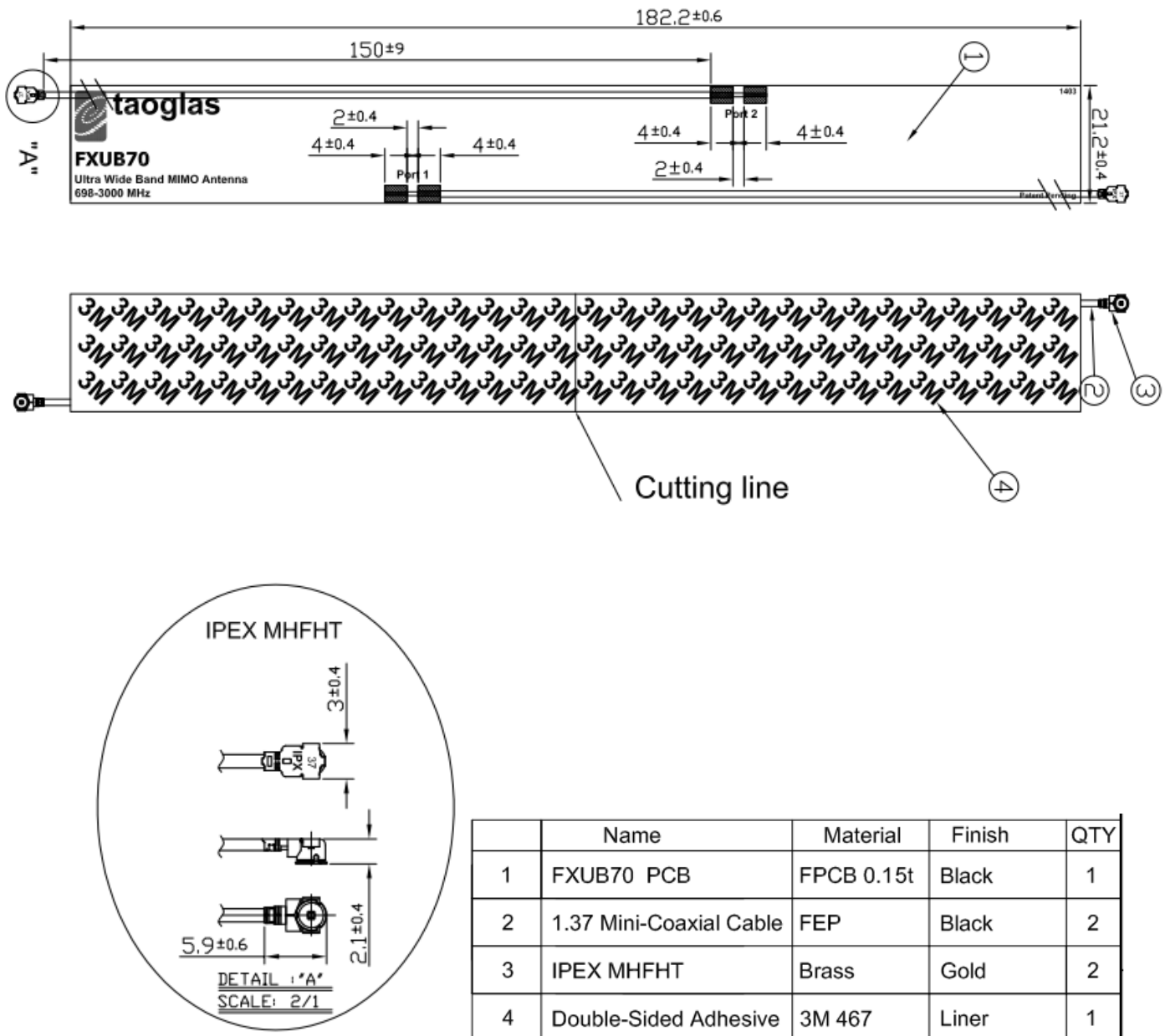
Figure 34. Mechanical drawing of FXUB70 UWB Antenna.
