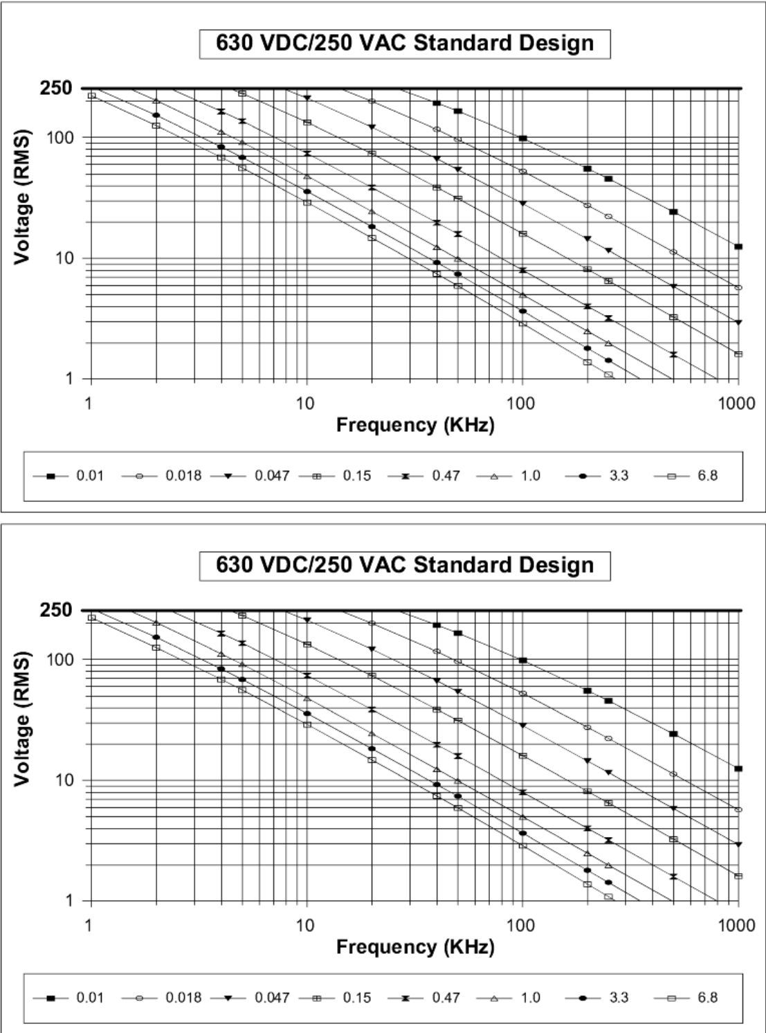
RMS Voltage vs. Frequency @ +85°C, in still air*
