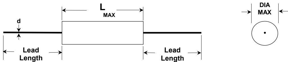
Wire Lead Termination (see lead length table below)
