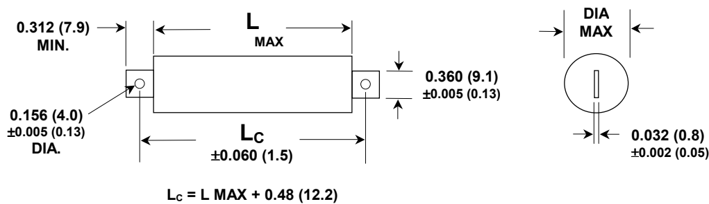
Wire Lead Termination (see lead length table below)
