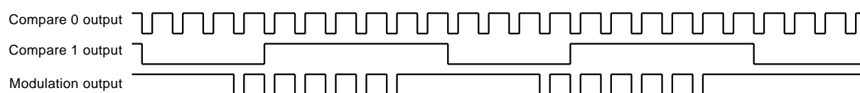
Fig. 48 Output compare mode (compare 0, 1 modulation mode: effect of output level latch)
