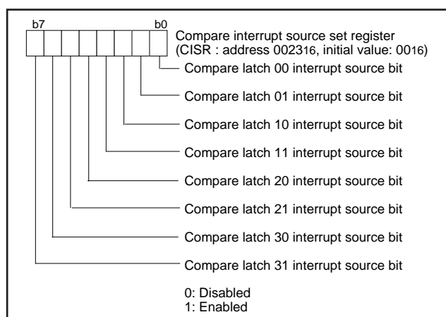
Fig. 41 Structure of compare interrupt source register
