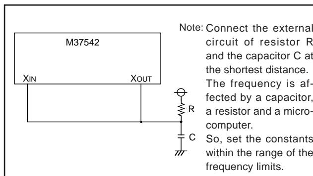
Fig. 78 External circuit of RC oscillation
