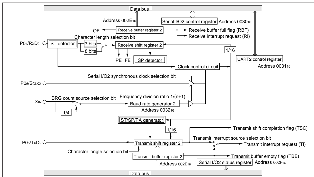
Fig. 65 Block diagram of UART serial I/O2
