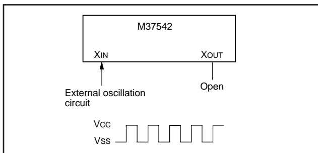
Fig. 79 External clock input circuit
