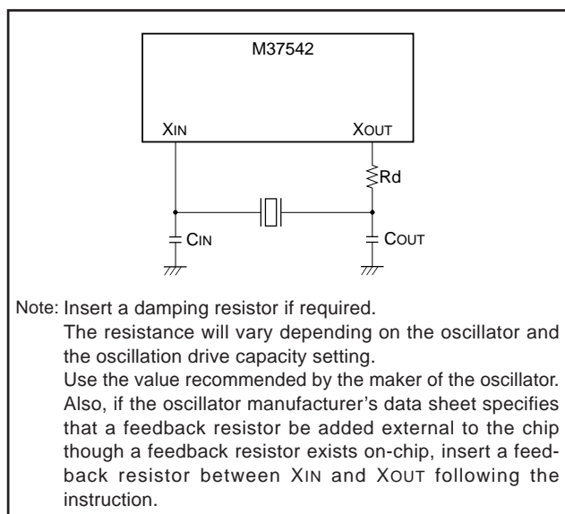
Fig. 77 External circuit of ceramic resonator
