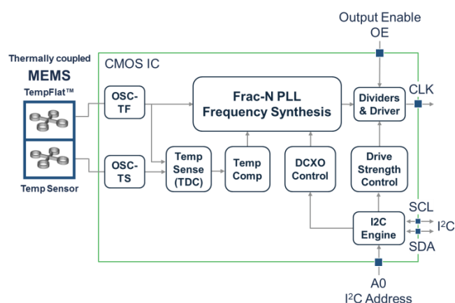
Figure 34. Block Diagram
