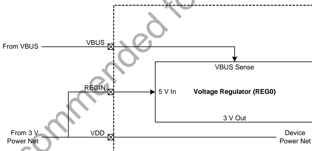
Figure 7.3. REG0 Configuration: USB Self-Powered, Regulator Disabled
