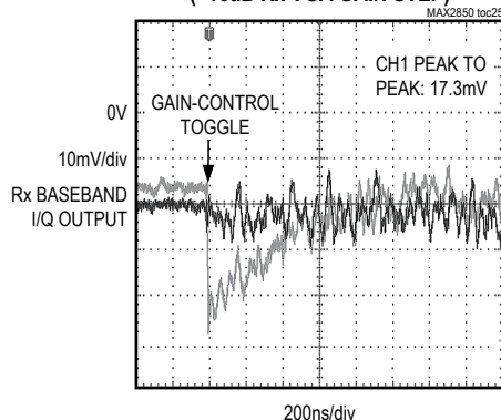
Rx DC OFFSET SETTLING RESPONSE (+16dB Rx VGA GAIN STEP)
