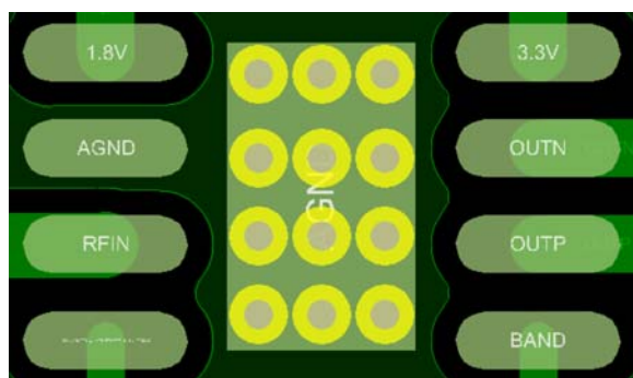
Figure 13. Evaluation Board Layout for the ADL5725 Package
