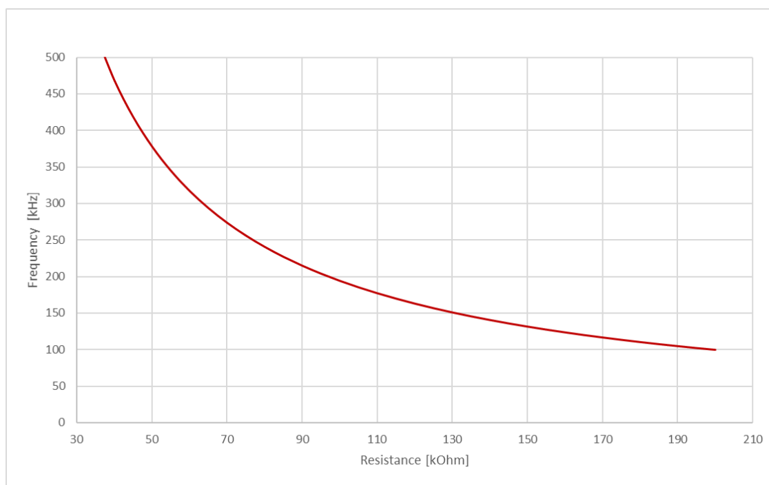
Figure 7.1. Switching Frequency vs R_{\text{FREQ}}
