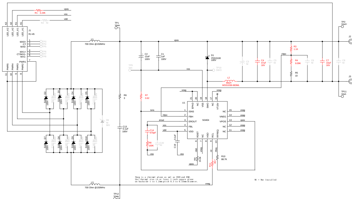
Figure 5.1. Si3404 Buck Non-Isolated EVB Schematic: 12 V, Class 3 PD
