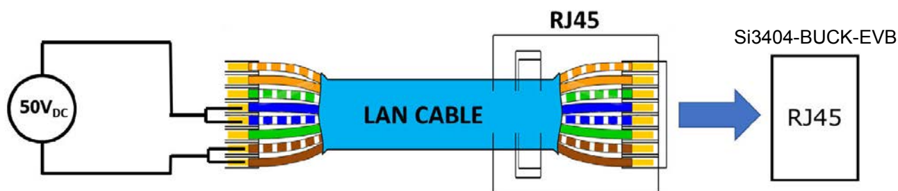
Figure 2.1. Endspan Connection using Laboratory Power Supply
