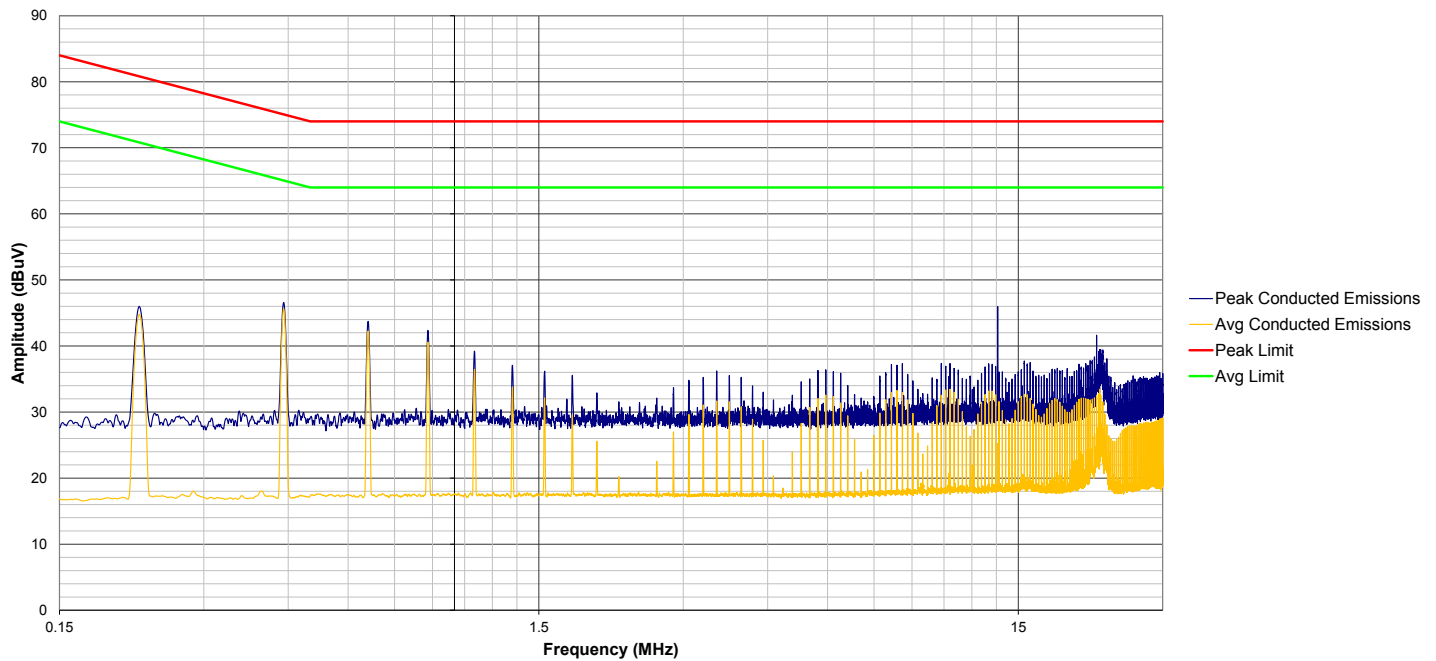
Figure 3.14. Si3404-Buck Non-Isolated EVB Conducted Emissions Measurements Results; 50 V Input, 3.3 V Output, 6.5 W Output Load
