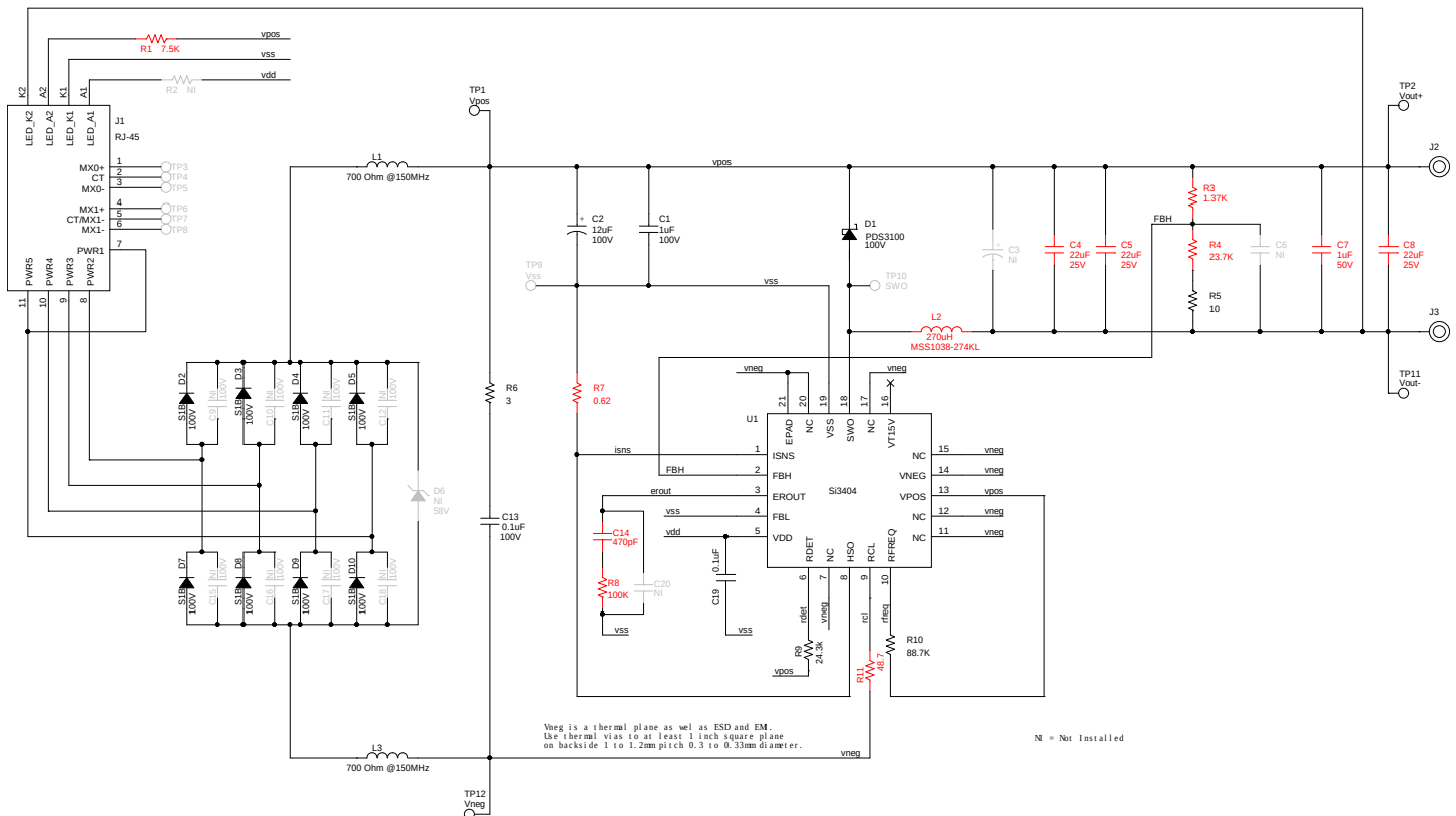
Figure 6.1. Si3404 Buck Non-Isolated EVB Schematic: 24 V, Class 3 PD
