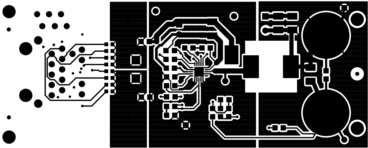
Figure 8.2. Top Layer
