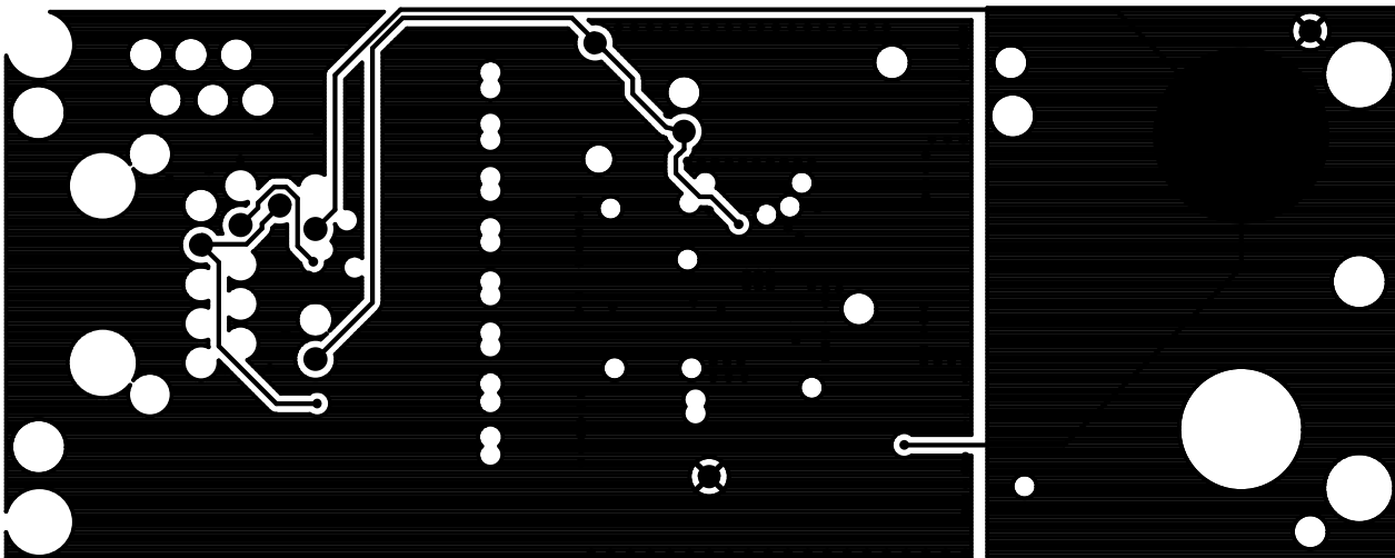
Figure 8.3. Internal 1 (Layer 2)
