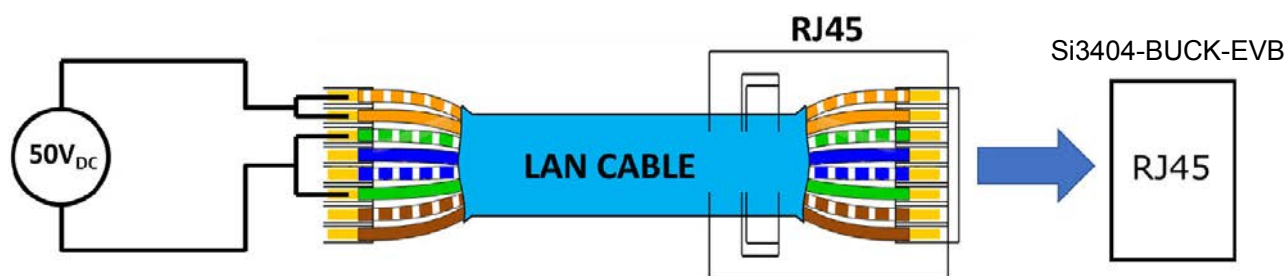
Figure 2.2. Midspan Connection using Laboratory Power Supply
