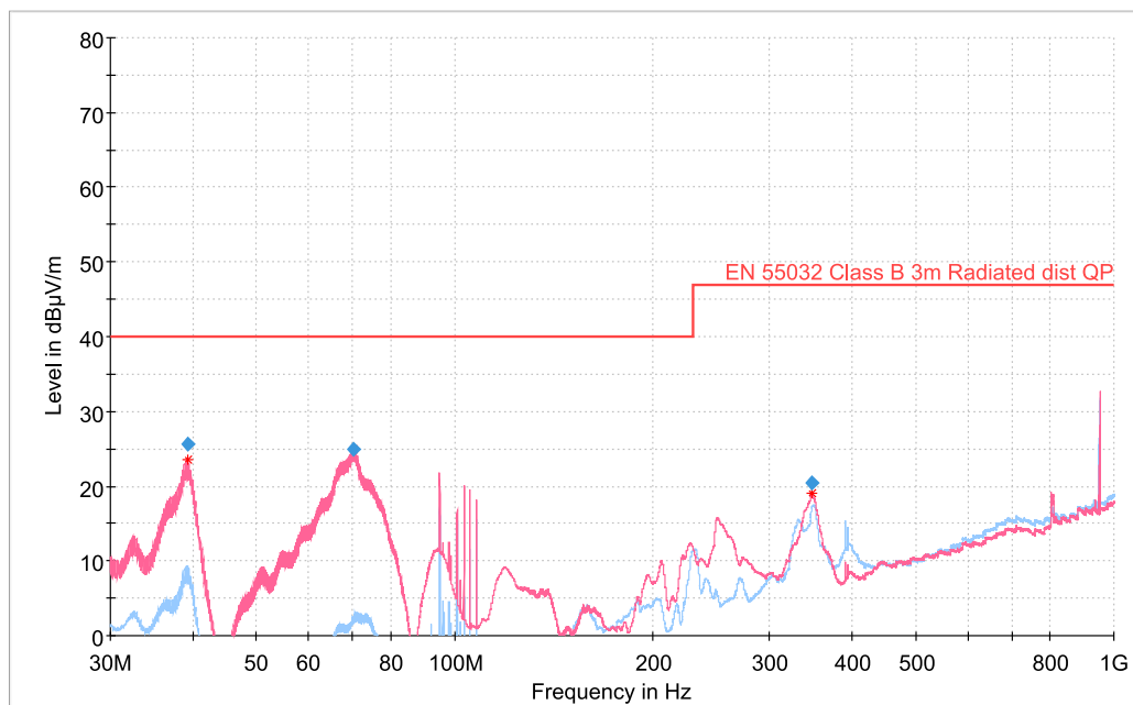
Figure 3.12. Si3404-Buck Non-Isolated EVB Radiated Emissions Measurements Results; 50 V Input, 3.3 V Output, 6.5 W Output Load
