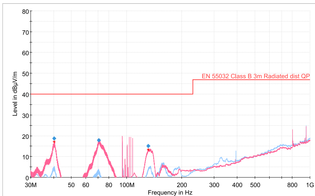
Figure 6.13. Si3404-Buck Non-Isolated EVB Radiated Emissions Measurements Results; 50 V Input, 24 V Output, 13 W Output Load
