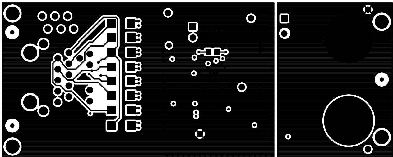
Figure 8.5. Bottom Layer
