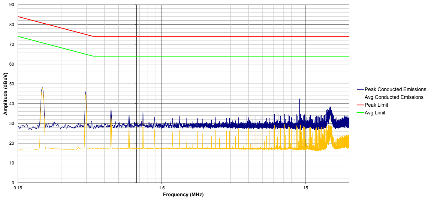
Figure 5.14. Si3404-Buck Non-Isolated EVB Conducted Emissions Measurements Results; 50 V Input, 12 V Output, 13 W Output Load
