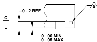
DETAIL "X"
