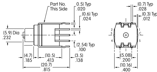
Terminals 1 & 5 are support pins
