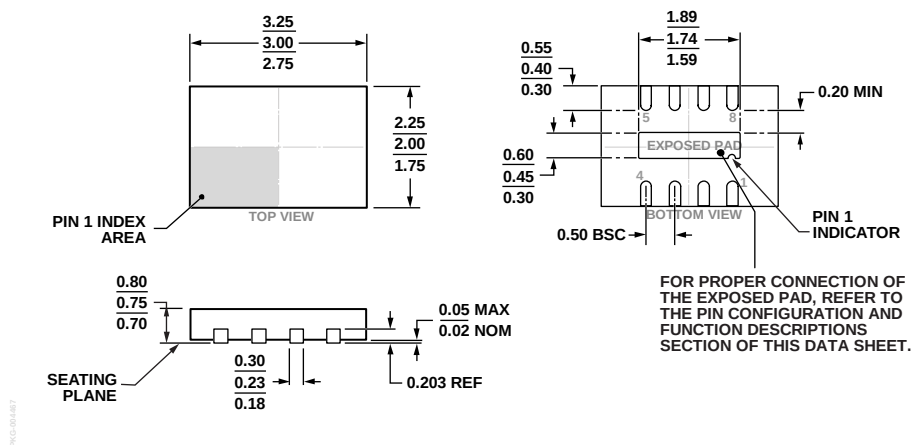
Figure 66. 8-Lead Lead Frame Chip Scale Package [LFCSP] 2 mm x 3 mm Body and 0.75 mm Package Height (CP-8-23) Dimensions shown in millimeters
