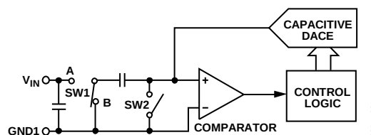
Figure 19. ADC Conversion Phase
