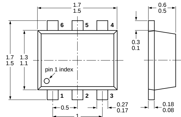
Fig 14. Package outline SOT666
