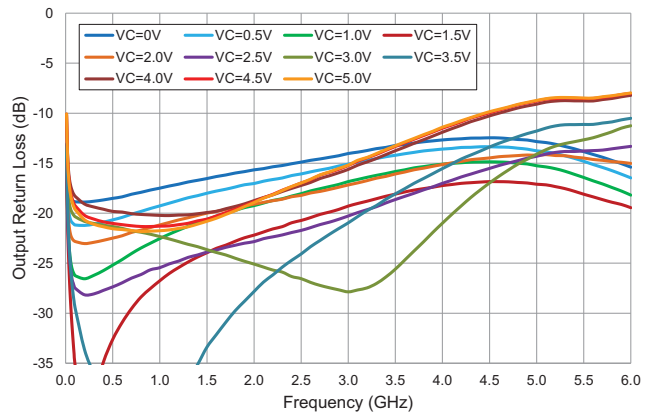
Output Return Loss versus Frequency V_{DD}=5V , Temp=+25°C
