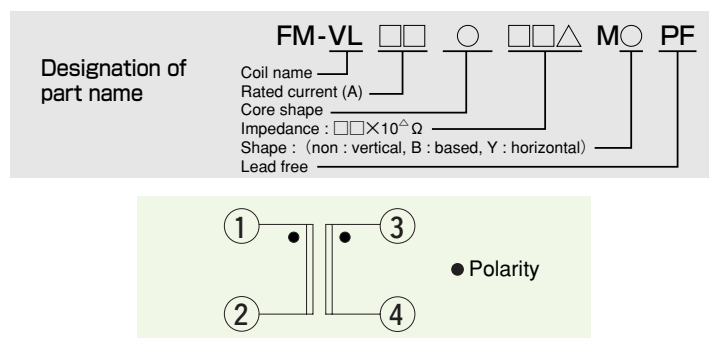
Figure 23. Circuit diagram
