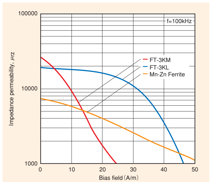
Figure 55. DC superposed characteristics of impedance permeability, \mu_r
